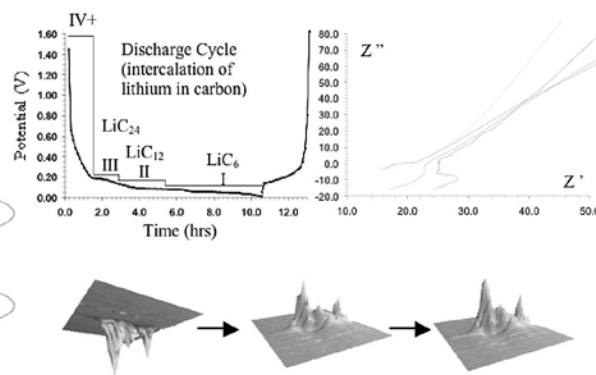
Figure 3. Overview of experiments performed with the two electrochemical-NMR/MRI imaging devices. Clockwise from top-left: galvanostatic cycling, electrochemical impedance spectroscopy, T 1 imaging.
