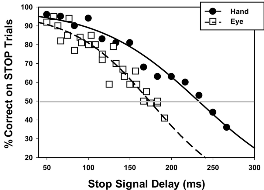
FIGURE 2 | STOP trial accuracy across various Stop Signal Delays during the oculomotor (dashed line) and manual motor (solid line) tasks. Data points represent mean performance across participants at each Stop Signal Delay for the eye (open square) and hand (closed circle). The gray horizontal line is shown to indicate the Stop Signal Delay at which individuals had a 50% probability of accurately inhibiting oculomotor (178 ms) and manual motor responses (227 ms). p_{50} values shown here are the means across subjects for each effector.
