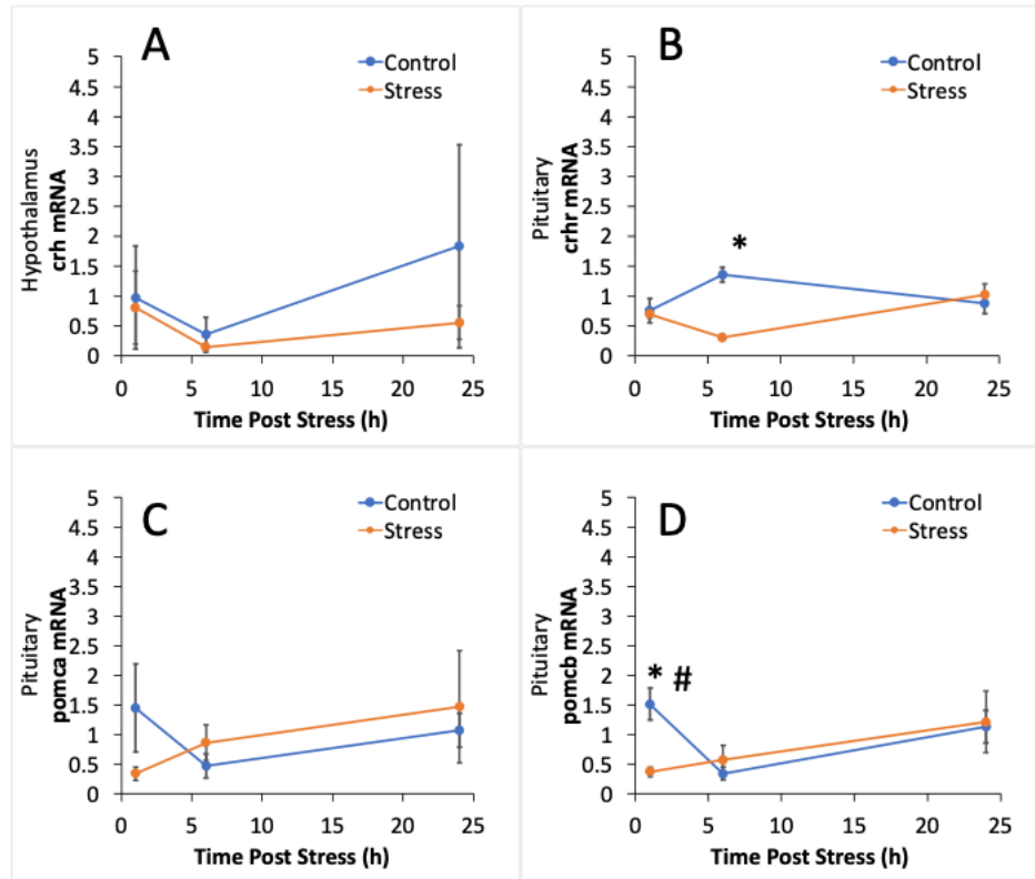
Fig. 2. Stress response in Atlantic sturgeon. mRNA concentrations in Atlantic sturgeon of crh in the hypothalamus (A), crhr in the pituitary (B), pomca in the pituitary (C), and pomcb in the pituitary (D) after 1, 6, and 24 h post stress. Data represent means \pm s.e.m. Asterisks indicates difference from control and stress at each respective time point. Pound symbol indicates difference from the mean control value.
