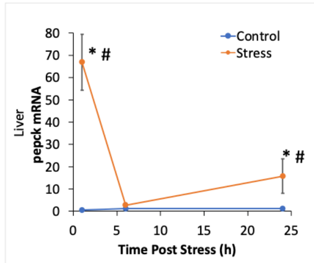
Fig. 4. Stress response in Atlantic sturgeon. mRNA concentrations in Atlantic sturgeon of pepck in the liver after 1, 6 and 24 h post stress. Data represent means±s.e.m. Asterisks indicates difference from control and stress at each respective time point. Pound symbol indicates difference from the mean control value.
