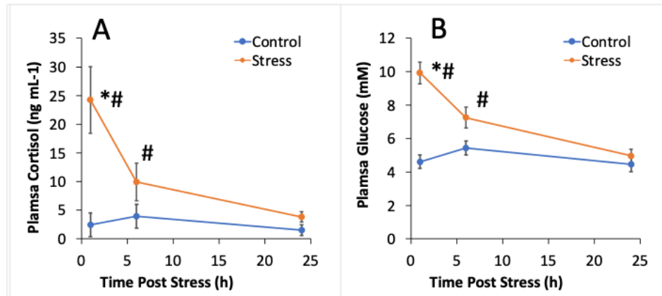
Fig. 1. Stress response in Atlantic sturgeon. Plasma concentrations of cortisol (A) and glucose (B) in Atlantic sturgeon at time 1, 6 and 24 h post stress. Data represent means \pm s.e.m. Asterisks indicates difference from control and stress at each respective time point. Pound symbol indicates difference from the mean control value.
