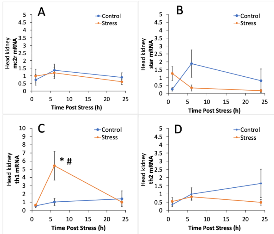
Fig. 3. Stress response in Atlantic sturgeon. mRNA concentrations in Atlantic sturgeon of mc2r in the head kidney (A), star in the head kidney (B), th1 in the head kidney (C), and th2 in the head kidney (D) after 1, 6 and 24 h post stress. Data represent means \pm s.e.m. Asterisks indicates difference from control and stress at each respective time point. Pound symbol indicates difference from the mean control value.
