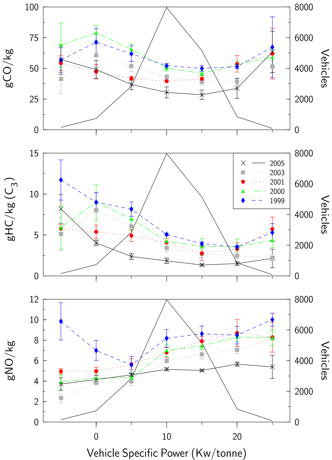
Figure 7. Vehicle emissions are plotted as a function of vehicle specific power for the entire Denver E-23 data sets. Error bars are standard errors of the mean calculated from daily samples. The solid line without markers is the vehicle count profile for the 2005 data set.
