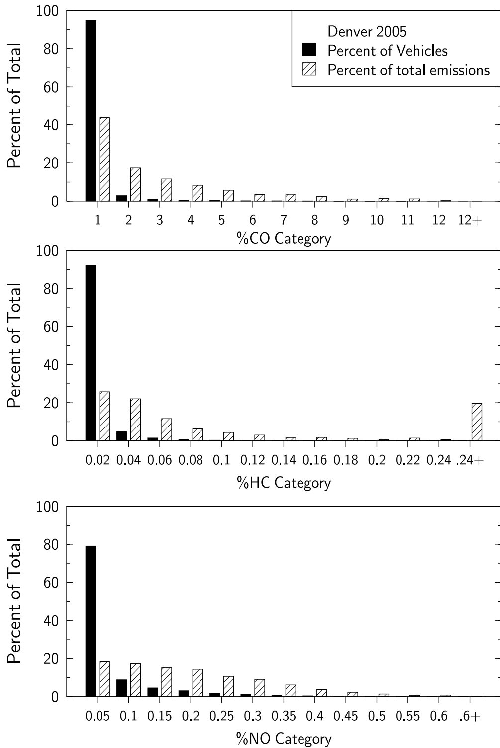
Figure 2. Emissions distribution showing the percentage of the fleet in a given emission category (black bars) and the percentage of the total emissions contributed by the given category (hatched bars).
