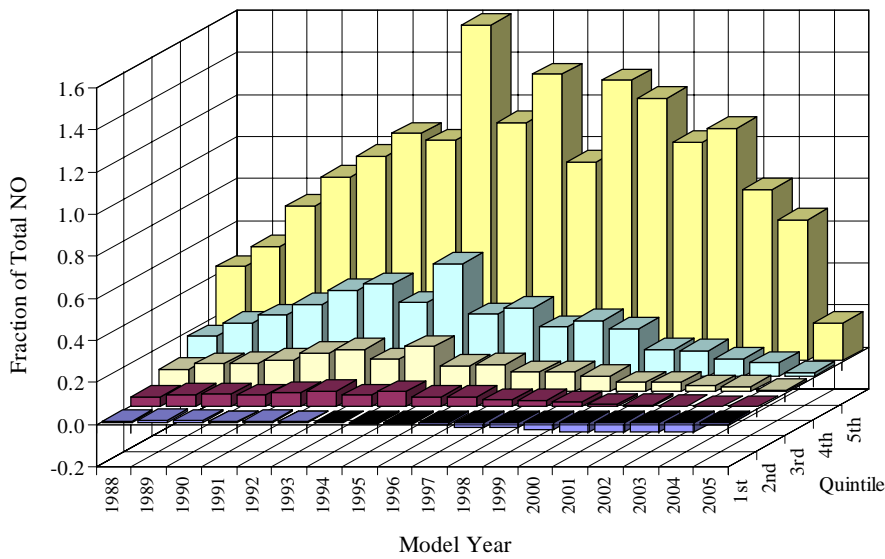
Figure 6. 2005 NO emissions by model year and quintile (top), fleet distribution (middle) and their product showing the total fractional NO emissions by model year and quintile (bottom).
