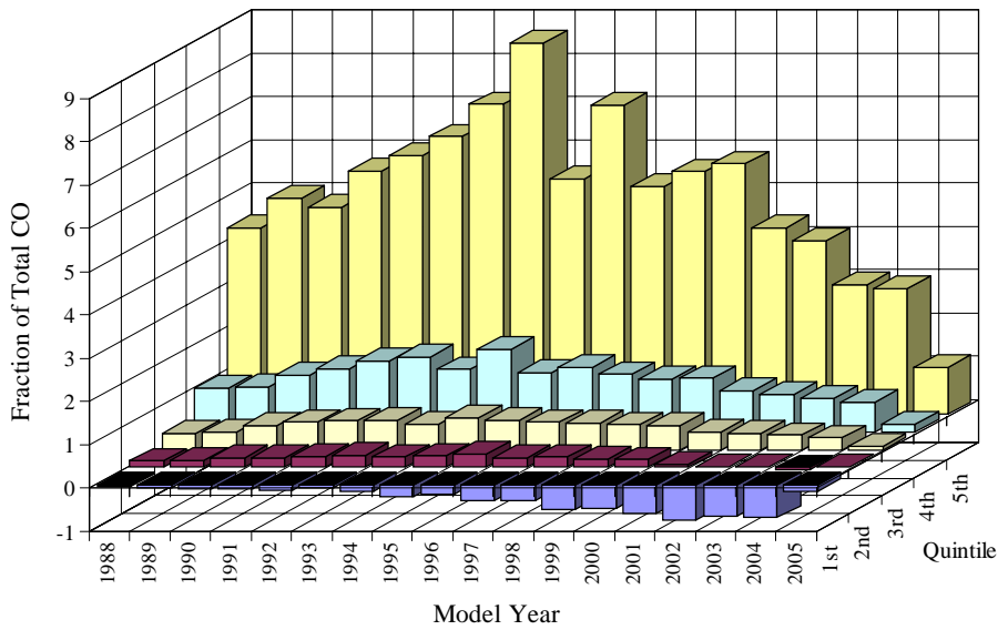
Figure 4. 2005 CO emissions by model year and quintile (top), fleet distribution (middle) and their product showing the total fractional CO emissions by model year and quintile (bottom).
