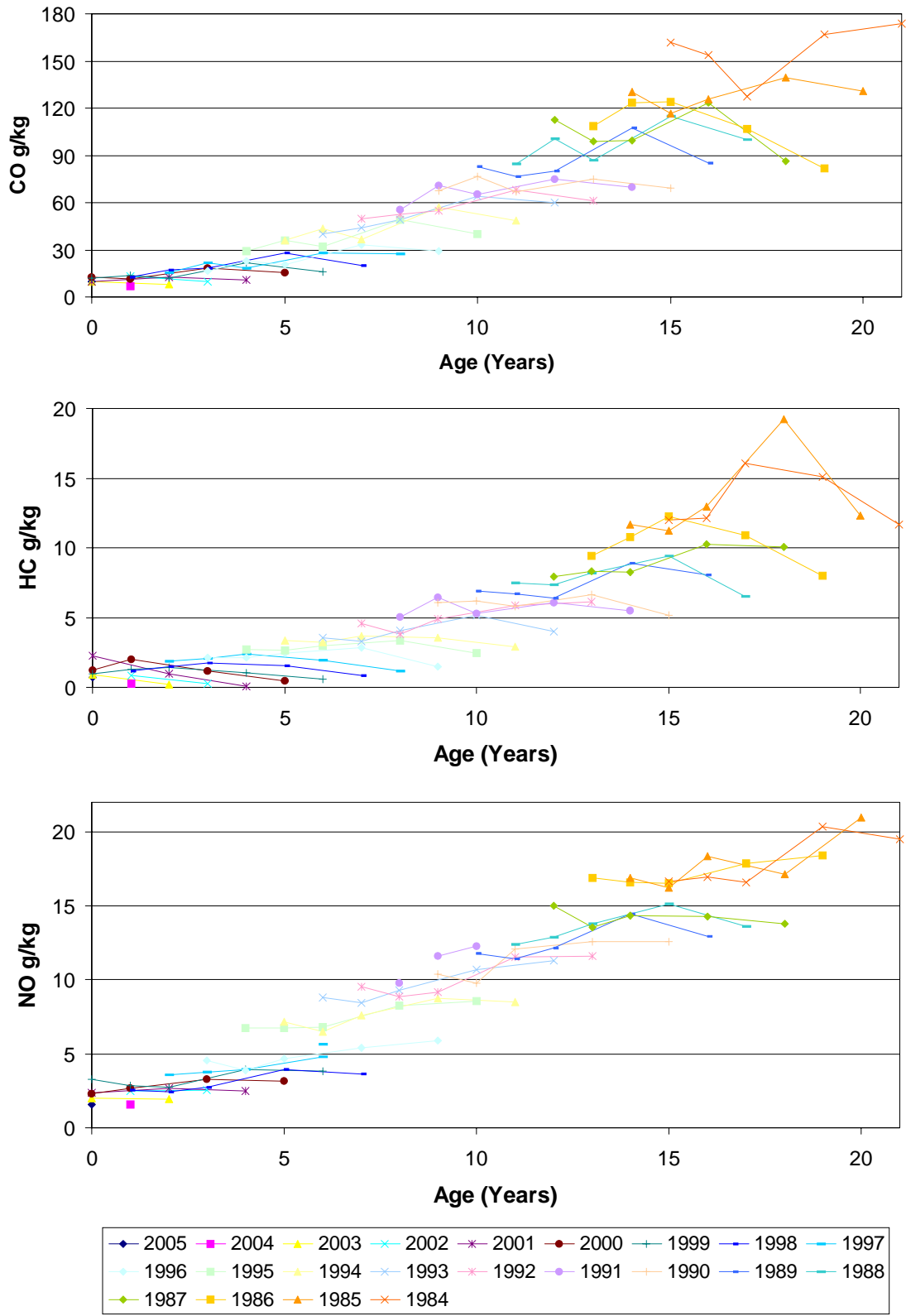
Figure 8. Mean vehicle emissions as a function of age, shown by model year. Included are data from the sites in 1999, 2000, 2001, 2003 and 2005.
