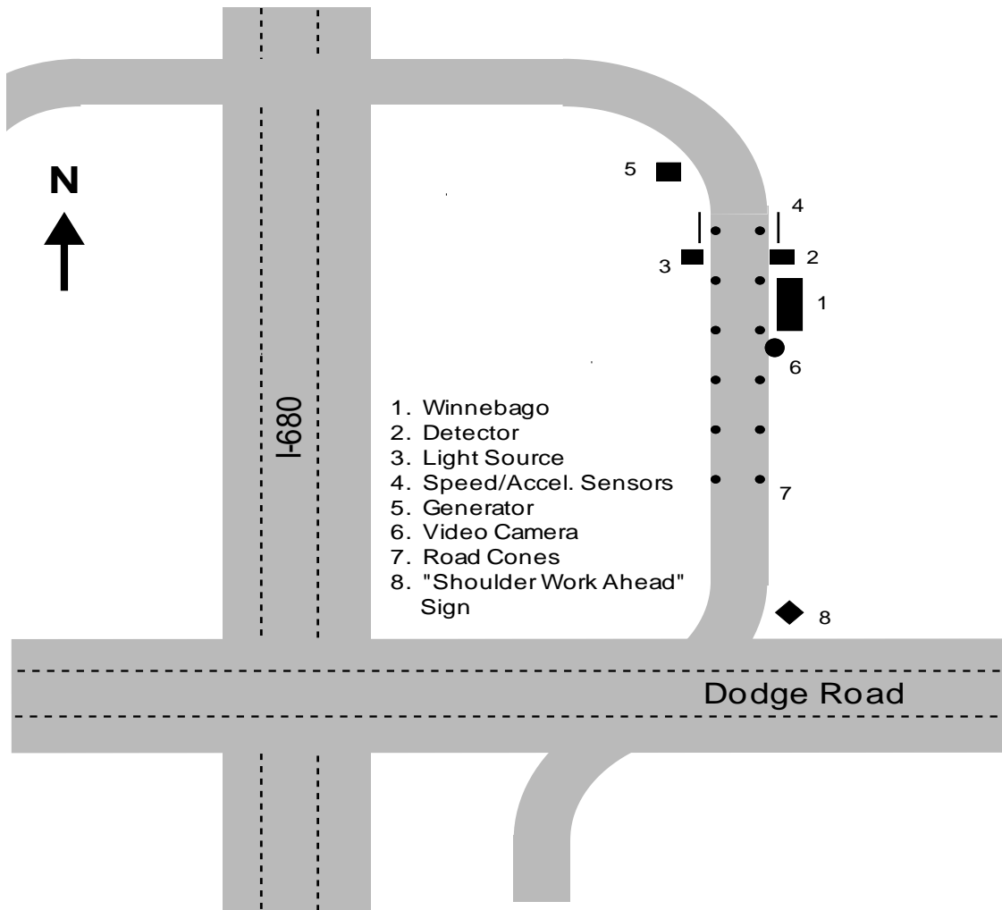
Figure 1. A schematic drawing of the ramp from westbound I-680 to westbound Dodge Rd. The location and safety equipment configuration was for all five days of measurements.
