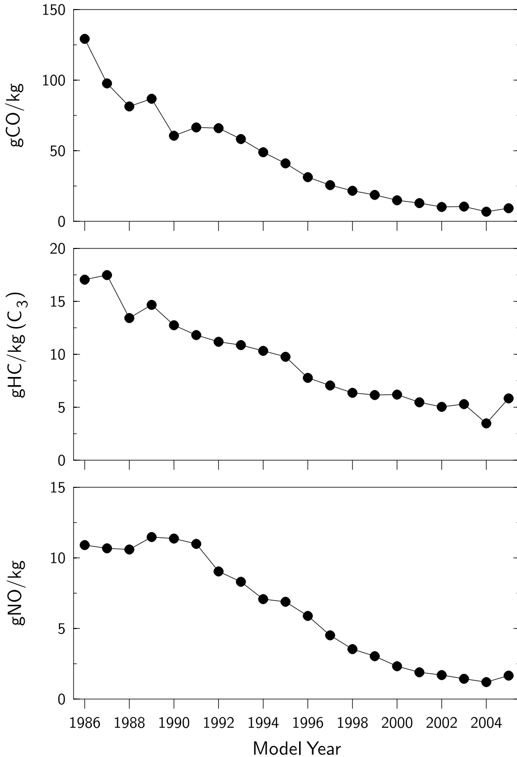
Figure 4. Mean vehicle emissions illustrated as a function of model year for the Omaha data set. HC data have been offset adjusted as described in the text.
