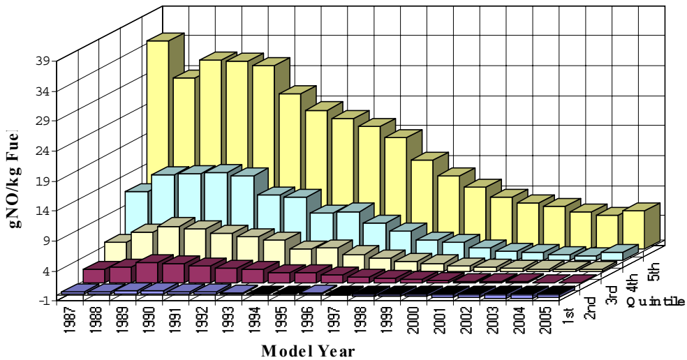
Figure 5. Vehicle emissions by model year for Omaha, divided into quintiles.
