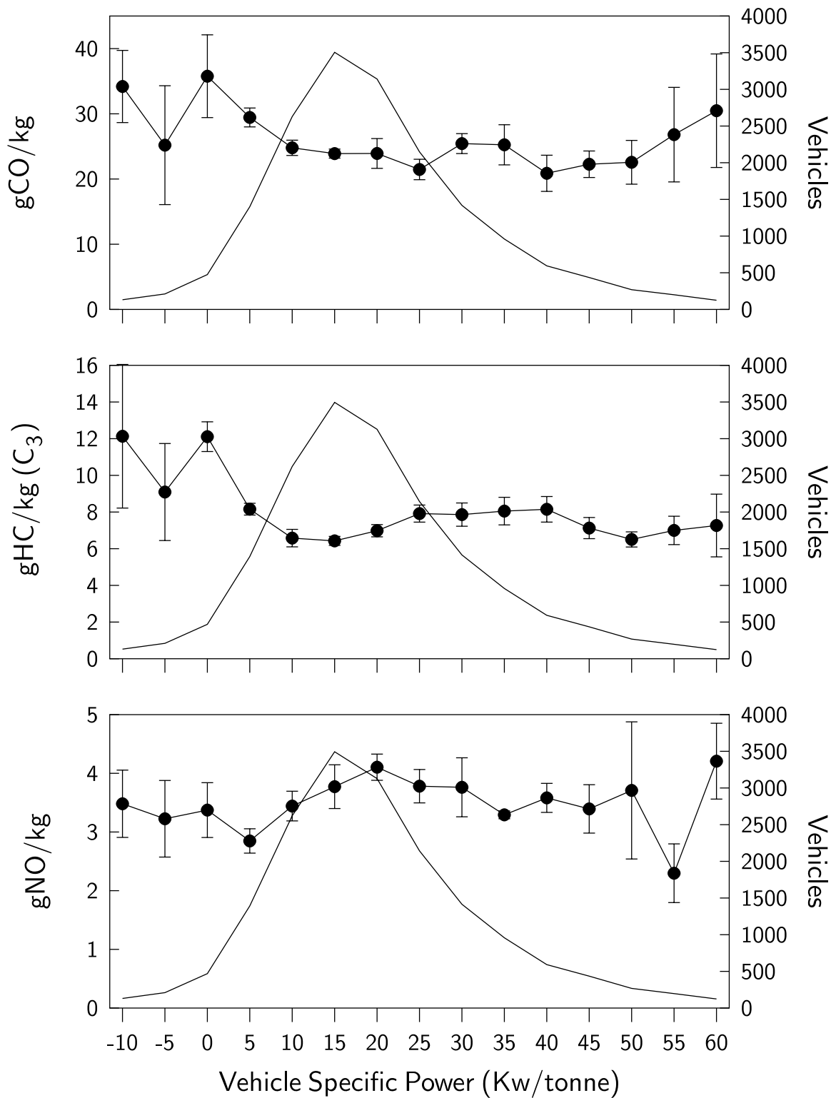
Figure 6. Vehicle emissions as a function of vehicle specific power for the Omaha data. Error bars are standard errors of the mean calculated from the daily samples. The solid line without markers is the vehicle count profile.
