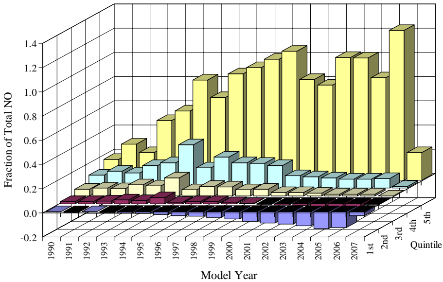
Figure 6. 2006 NO emissions by model year and quintile (top), fleet distribution (middle) and their product showing the total fractional NO emissions by model year and quintile (bottom).
