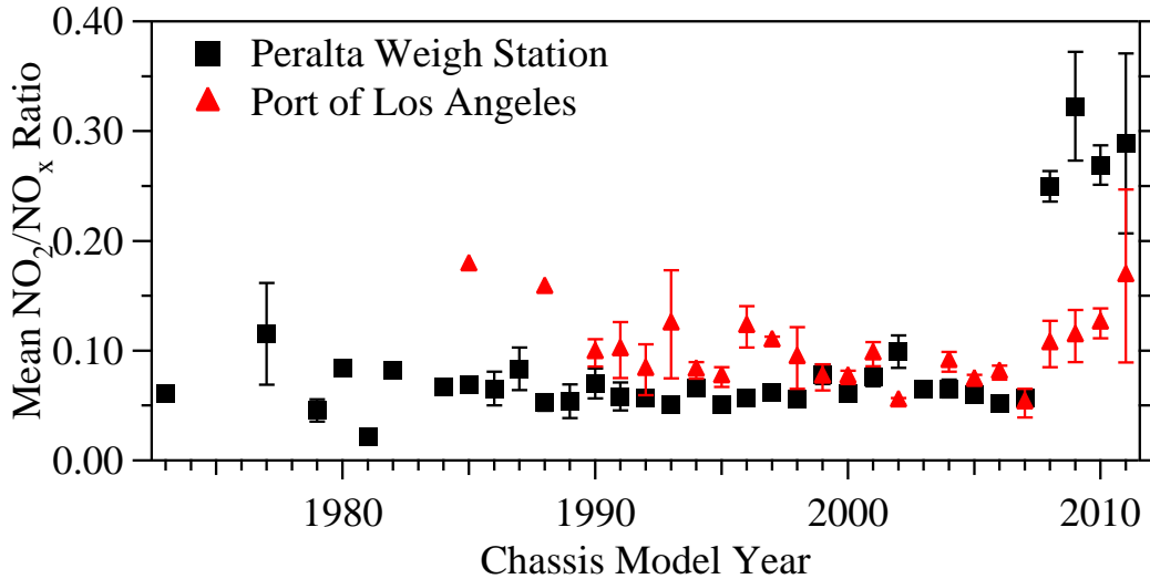
Figure 10. Ratio of NO 2 /NO x vs. chassis model year for HDDV's at each site. New technologies implemented to meet new EPA standards yield higher proportions of NO 2 in MY 2008-2011 trucks. Uncertainties are standard errors of the mean.
