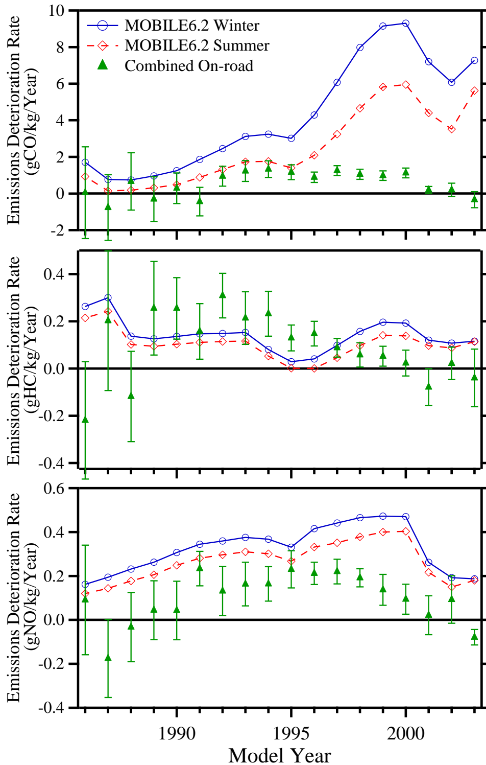
Figure 5. On-road emissions deterioration rates (see Figure 4) versus model year compared with emissions deterioration rates determined from the U.S. EPA’s MOBILE6.2 vehicle emissions computer model. The uncertainty bars plotted with the on-road data are the standard error of the slope for the least squares fit. The MOBILE6.2 grams/gallon data have been converted to g/kg assuming a fuel density of 726 grams/liter and the MOBILE6.2 NO 2 emissions have been converted to NO equivalents for comparison with the on-road data.
