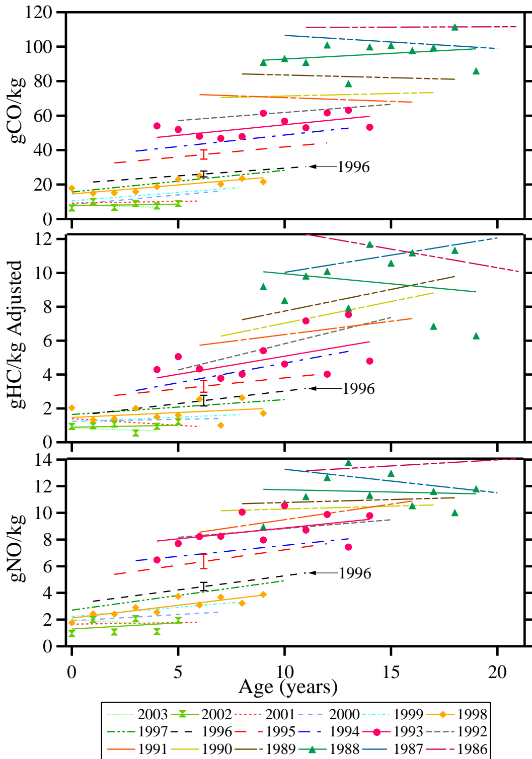
Figure 4. Linear least square fits to mean, fuel specific vehicle emissions as a function of age from the combined data of Chicago, Denver, West LA and Phoenix. The data are grouped by model year beginning with 2003, which is the first model with at least three measurements, and go back to the 1986 model year. The data used to construct the linear fits are displayed for model years 2002, 1998, 1993 and 1988. The error bars plotted for model years 1995 and 1996 are 95% confidence limits for the midpoints.
