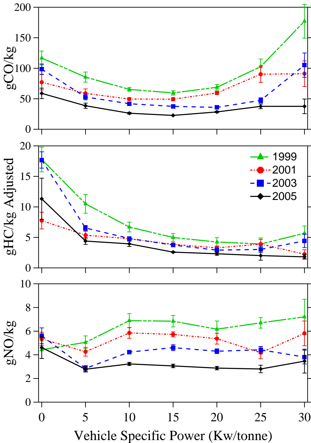
Figure 3. Mean, fuel specific emissions for the four years of data collected at the West LA site plotted as a function of Vehicle Specific Power. Only emissions data with valid speed and acceleration measurements are plotted and the uncertainties displayed are standard errors of the means calculated using the daily means.
