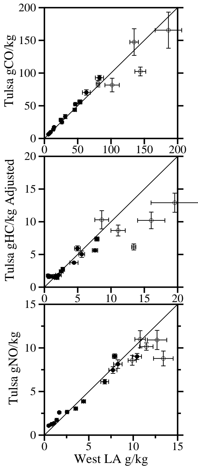
Figure 6. Fuel specific emissions comparison between the 2003 data sets collected in Tulsa, OK and West Los Angeles, CA for model years 2003 to 1986. The uncertainty bars plotted are standard errors of the mean calculated from the daily means at each site. The 1:1 line is plotted as a reference. 1990 to 1986 model years (open circles) with the most noticeable uncertainty bars constitute less than 12% of the West LA fleet and less than 6% of the Tulsa fleet.
