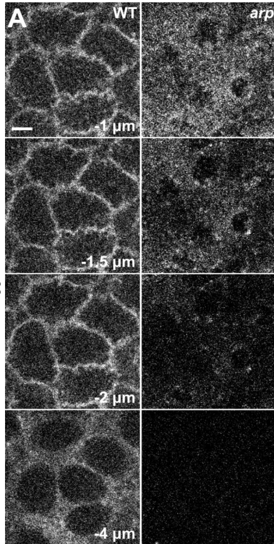
Figure 5. Arp2/3 is required for syncytial furrow ingress. (A) Still images from live-imaging furrow dynamics at t=4 min in cycle 12 in wild-type and arpc4 embryos. (B) Biphasic furrow ingress dynamics in wild-type and arpc4 embryos from cycle 10-13.
