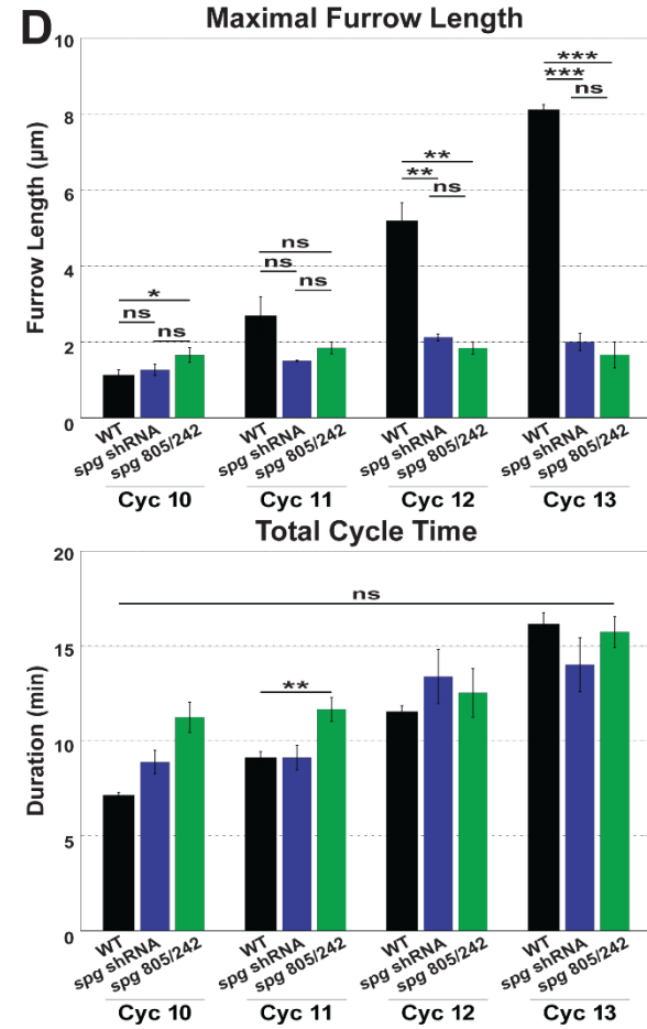
Figure 1 cont. Spg is required for syncytial furrow ingression. (C) Biphasic furrow ingression dynamics in wild-type, spg shRNA, and spg mutant embryos from cycle 10-13. (D) Maximal furrow length and total cycle time from cycle 10-13.
