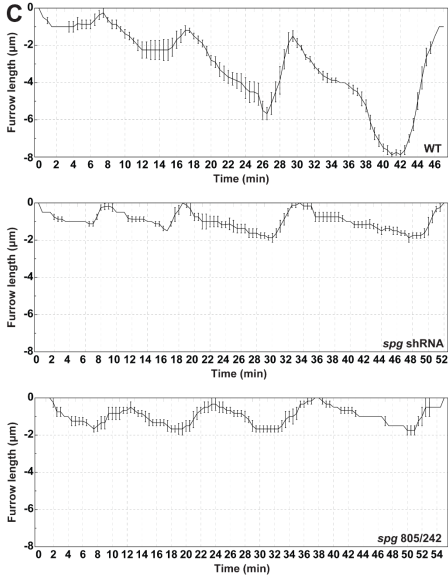
Figure 1 cont. Spg is required for syncytial furrow ingression. (C) Biphasic furrow ingression dynamics in wild-type, spg shRNA, and spg mutant embryos from cycle 10-13. (D) Maximal furrow length and total cycle time from cycle 10-13.
