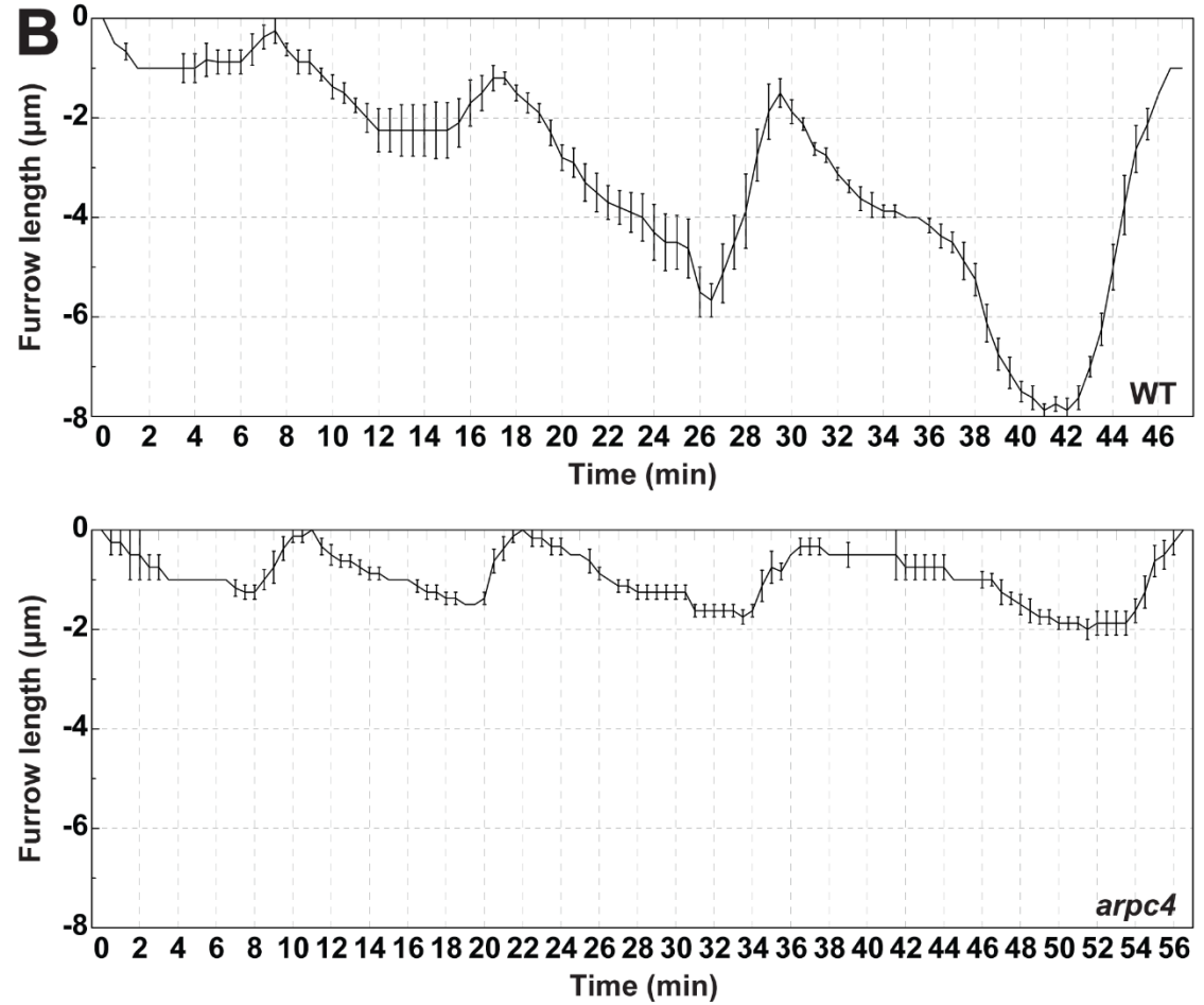
Figure 5. Arp2/3 is required for syncytial furrow ingress. (A) Still images from live-imaging furrow dynamics at t=4 min in cycle 12 in wild-type and arpc4 embryos. (B) Biphasic furrow ingress dynamics in wild-type and arpc4 embryos from cycle 10-13.
