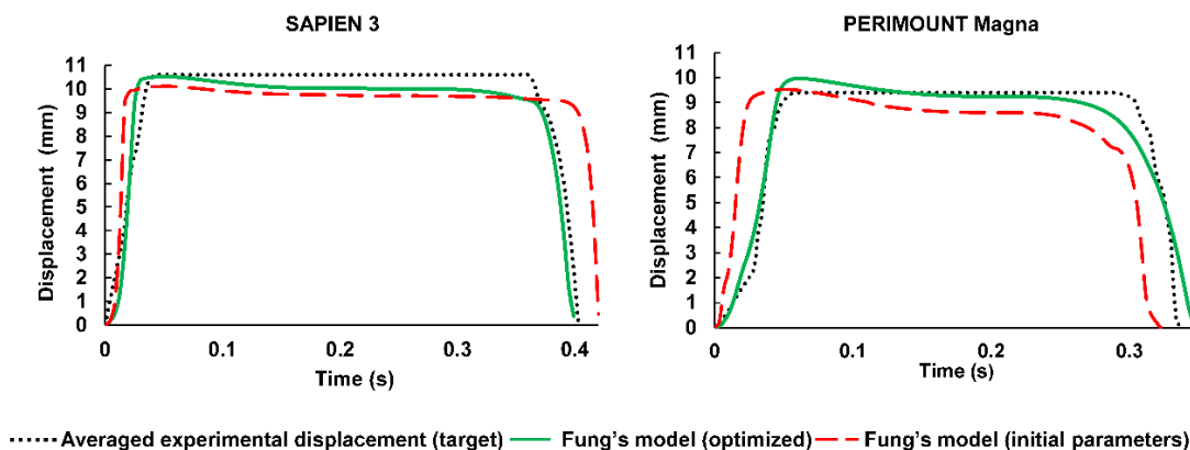
..... Averaged experimental displacement (target) — Fung's model (optimized) - - Fung's model (initial parameters) Figure 15- Optimization results for the averaged leaflet tip displacement for each valve. Each graph compares the optimized FE simulations with the experimental data and simulation with initial parameters
