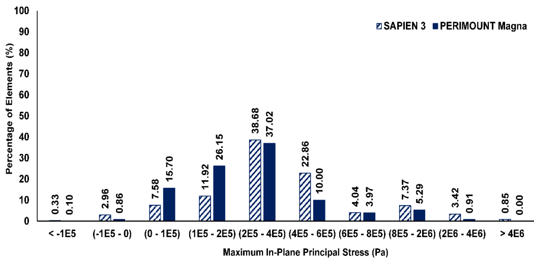
Figure 22-Distribution of maximum in-plane principal stress at peak systole at each node for each valve
